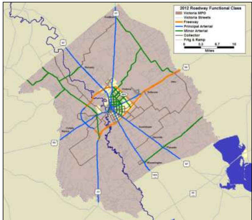
Figure 3.15: 2012 Functional Class, City of Victoria
