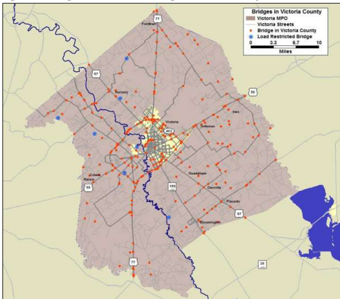
Figure 2.1: Bridges and Load Posted Bridges in Victoria County
