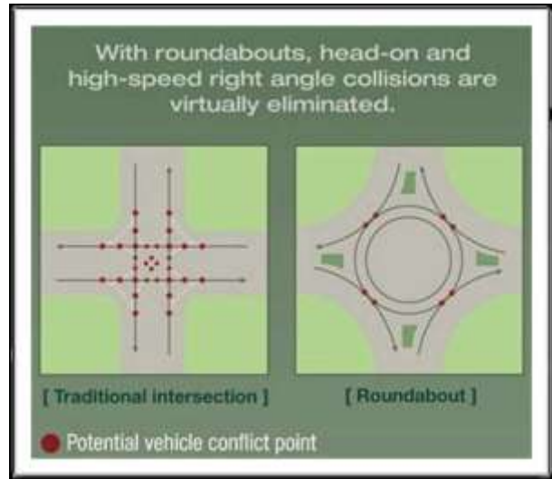
Figure 6.5: Standard Intersection and Roundabout
