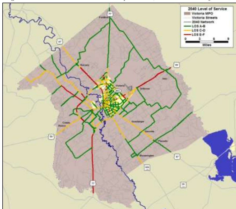
Figure 3.19: 2040 Network Level of Service, Victoria County
