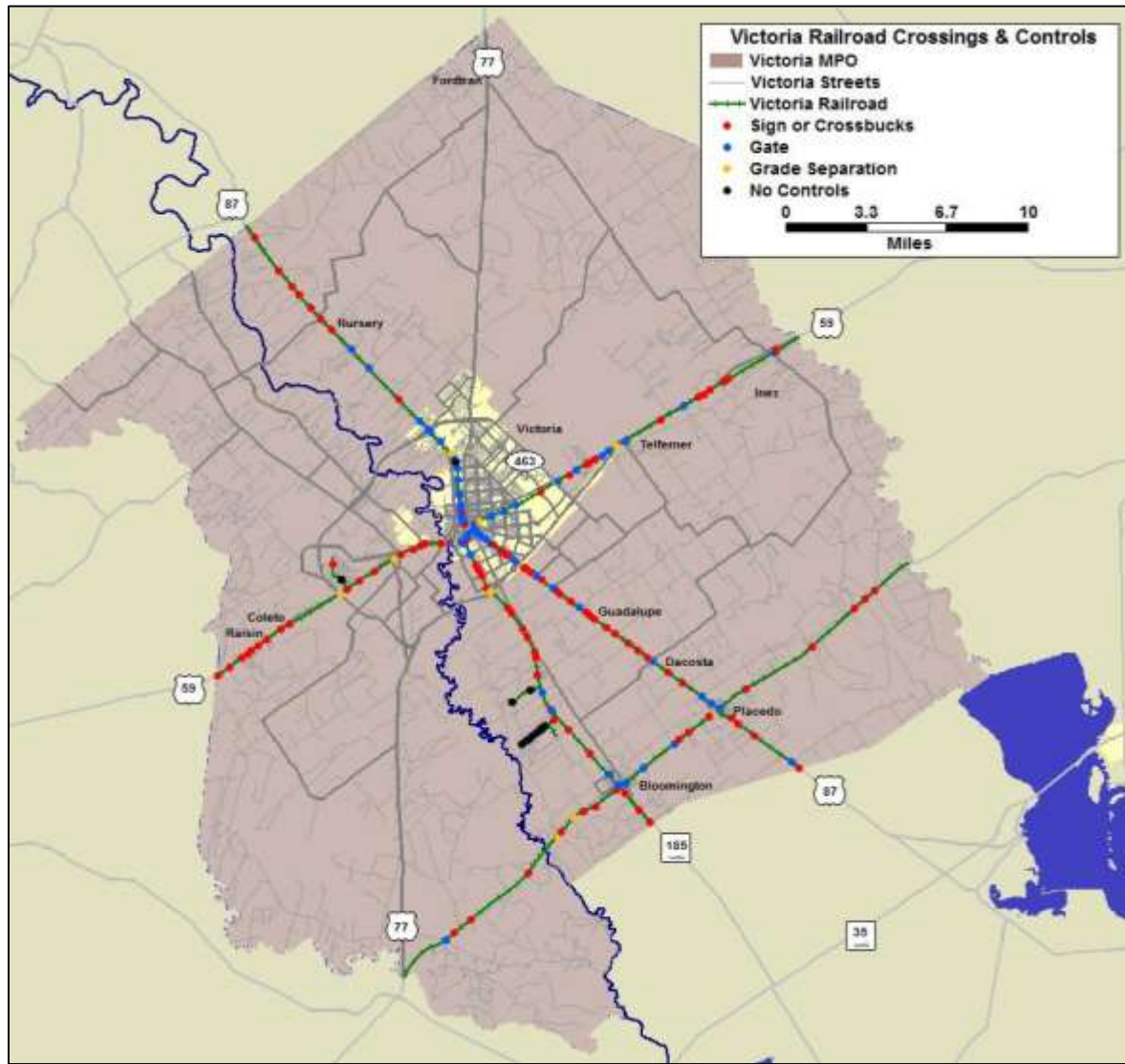
Figure 6.19: Railroad Crossings and Controls
